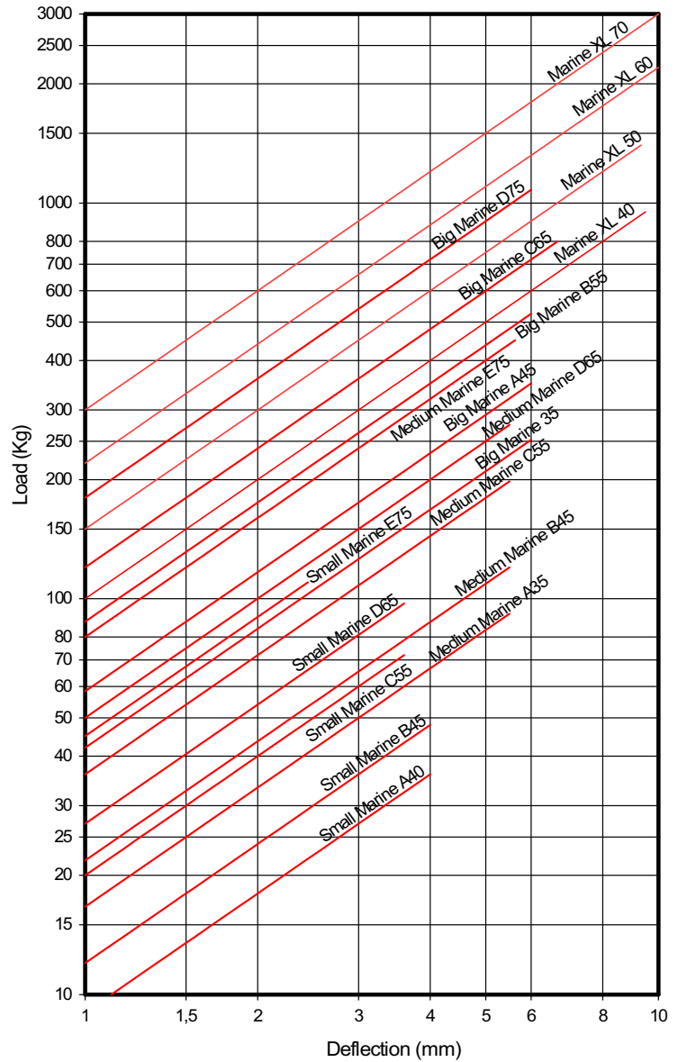
LOAD DEFLECTION GRAPHS AMC MECANOCAUCHO® Type Marine
